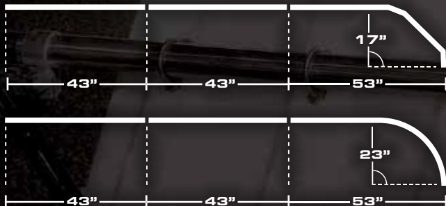
FENDER WIDTH: 25.5"
